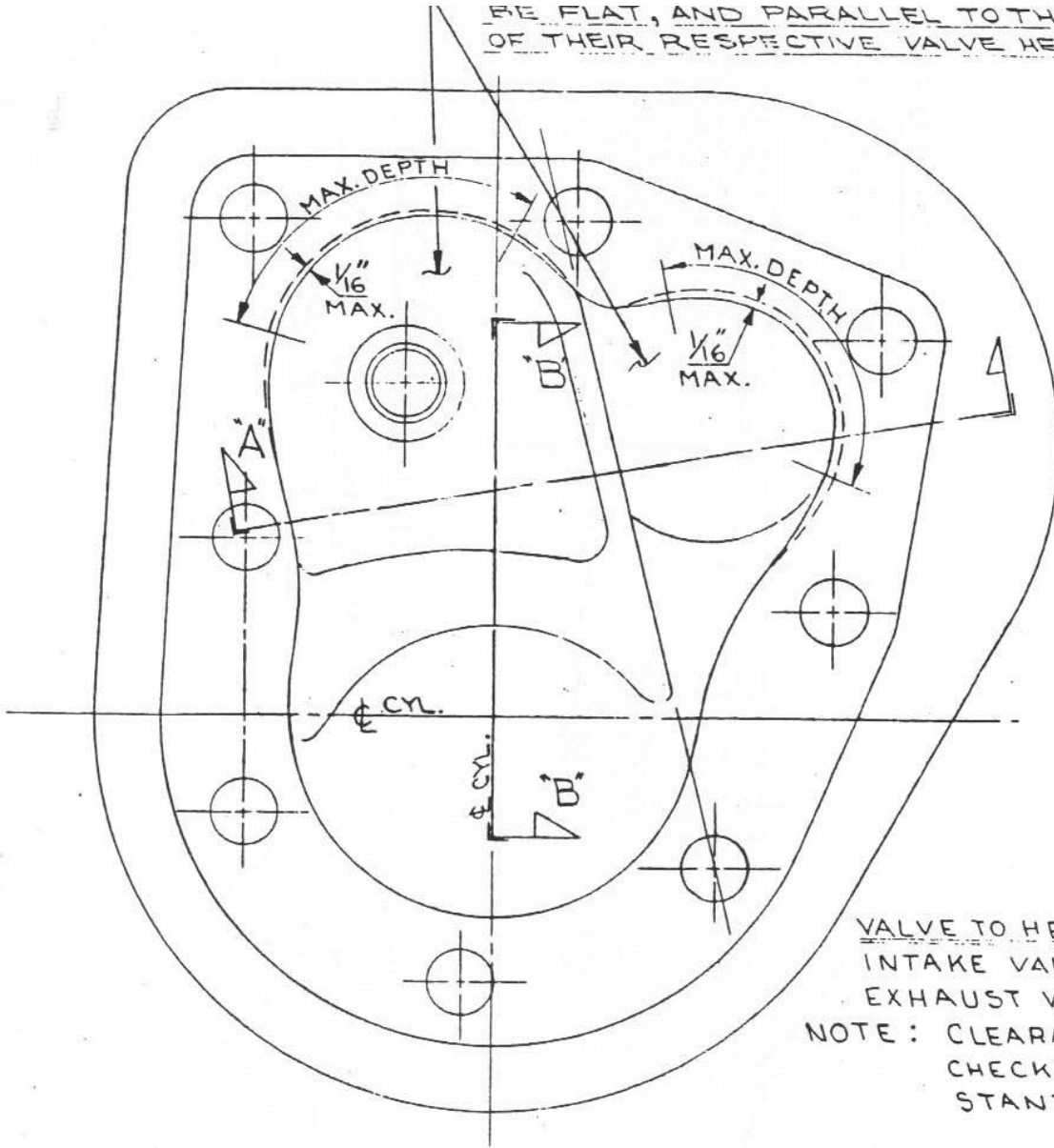
BOTTOM VIEW
