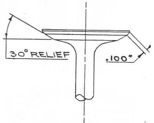
EXHAUST VALVE
