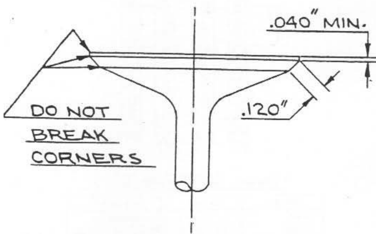
INTAKE VALVE
