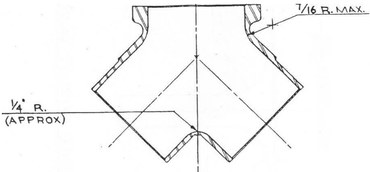
KR INTAKE MANIFOLD
